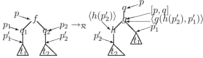
Figure 1: An idea of automata construction.
